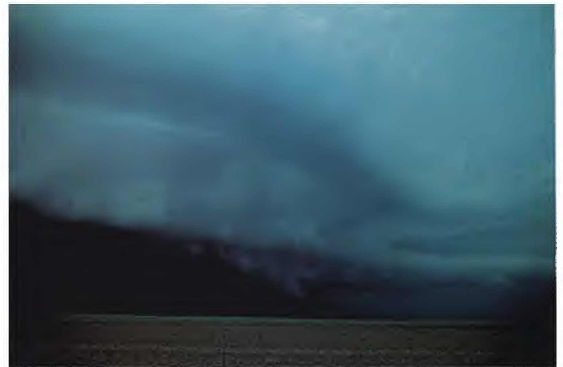
Figure 20: A beaver’s tail is seen extending to the right of the main updraft tower. View is to the north. Photo - Alan Moller.
